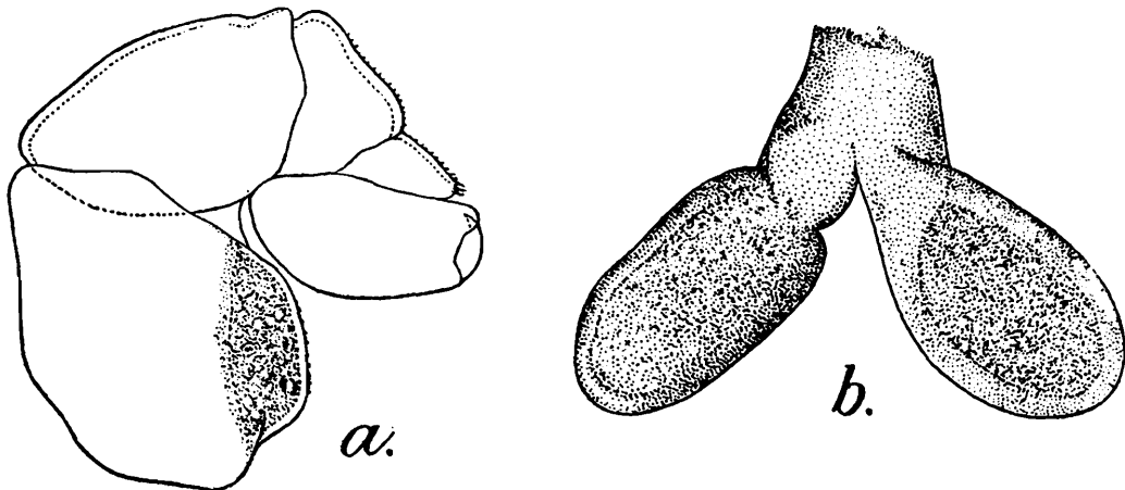
TEXT-FIG. 20.— Palaegyge pica , sp. nov. a. Thoracic leg of female : \times 100 . b. Pleopod : \times 100 .
