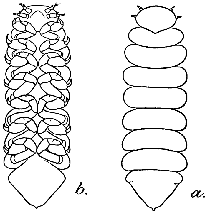
TEXT-FIG. 6.— Epipenaeon elegans , sp. nov. Type-specimen, male. a. Dorsal view: \times 12 . b. Ventral view: \times 12 .
