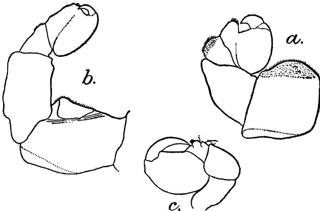
TEXT-FIG. 8.— Stegoalpheon kempfi , sp. nov.
